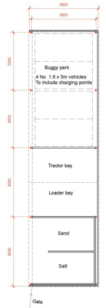
Plan of utility shelter 1:100
